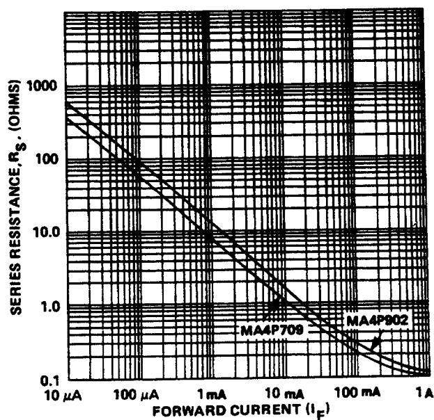
FORWARD CURRENT vs SERIES RESISTANCE (MA4P709, MA4P902)
