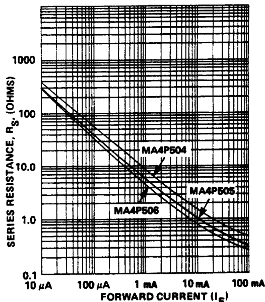
FORWARD CURRENT vs SERIES RESISTANCE (MA4P504, MA4P505, MA4P506)
