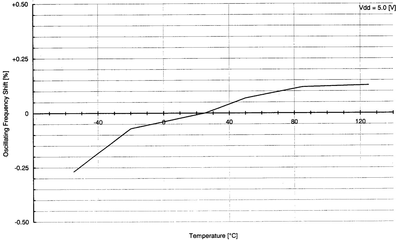
Temperature Characteristics of Oscillating Frequency MODEL : CSTCC8.00MG with M34580E4
