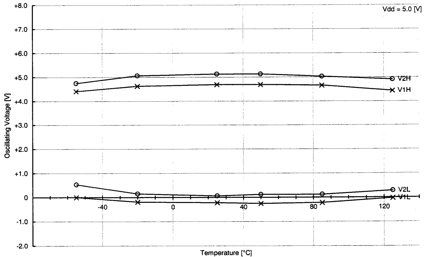
Temperature Characteristics of Oscillating Voltage MODEL : CSTCC8.00MG with M34580E4
