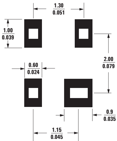
Dimensions in \frac{\text{mm}}{\text{inches}}
