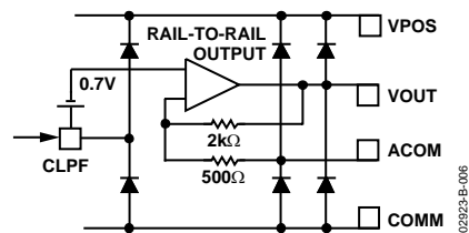
Figure 6. Circuit D
