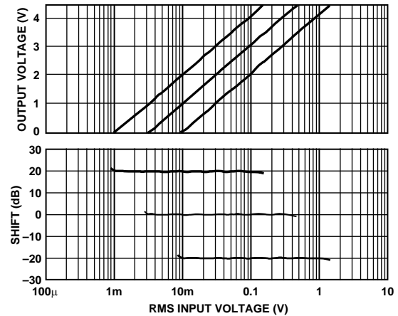
Figure 66. Illustrative Results for Slope of 100 mV/dB
