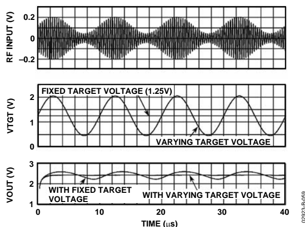
Figure 59. Waveforms for Envelope Elimination Scheme
