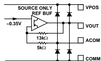
Figure 7. Circuit E
