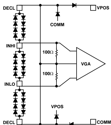
Figure 3. Circuit A
