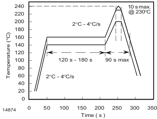
Figure 3. Recommended Solder Profile for Sn/Pb soldering
