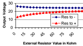
PM2024D12 Voltage Trim Adjusts the total voltage (+) out to (-) out
