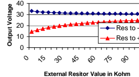
PM2024D15 Voltage Trim Adjusts the total voltage (+) out to (-) out
