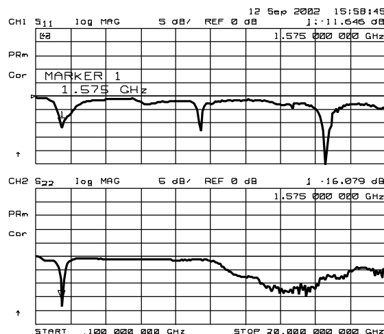
S11, S22(~20GHz)
