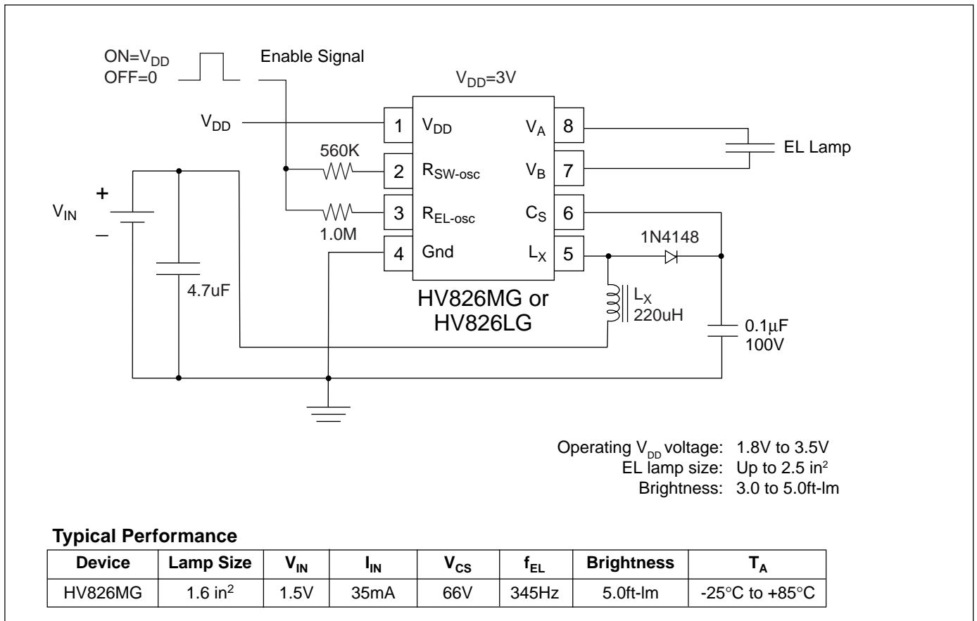
Figure 1: Typical Application
