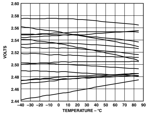
TPC 24. Typical Y-Axis Zero g Output vs. Temperature for 16 Parts
