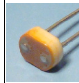
LDR 2856K / 10lux, R = 5 - 10k, pimeäres. minimi 300k, Ø 6mm/7mm
